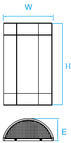
Model No. KLW043 Dimension 8-7/8"W x 14"H x 3-1/2"E Lamp (2) medium or GU24 base 16W integral LED 1100 lumens
