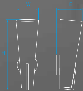
Model No. KLW193 Dimension 5"W x 15-1/2"H x 5-3/4"E Lamp 15W integral LED 900 lumens
