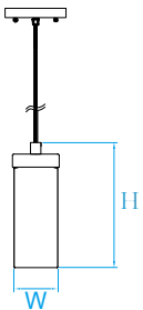
Model No. KLP181 Dimension 3-1/2"W x 8"H Lamp (1) medium or GU24 base
