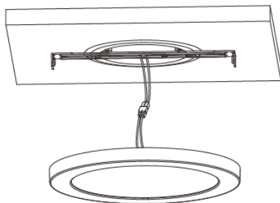
J-BOX Mount
